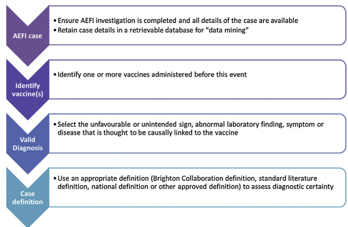
Fig. 1. Eligibility criteria for tool application. Brighton collaboration [22].
